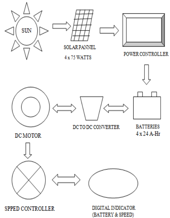
Fig:1 working Diagram of Solar Vehicle
